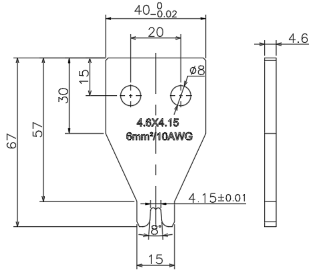
Crimping Tool Drawing (Fig 12&13)
